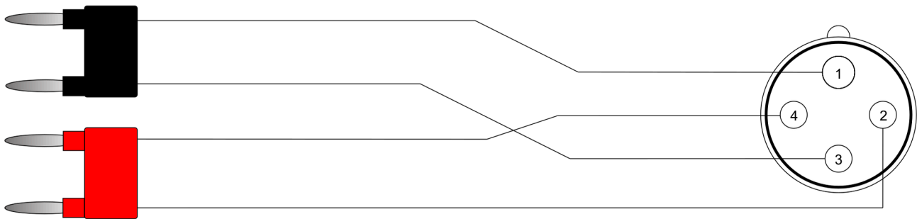
Comms Rope Wiring
