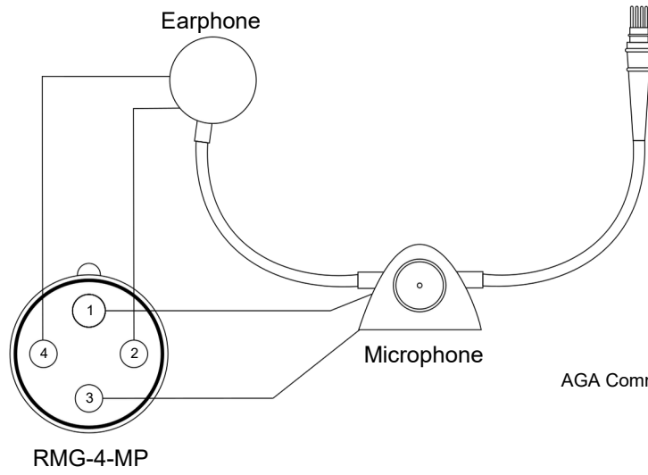
Comms Rope Wiring
